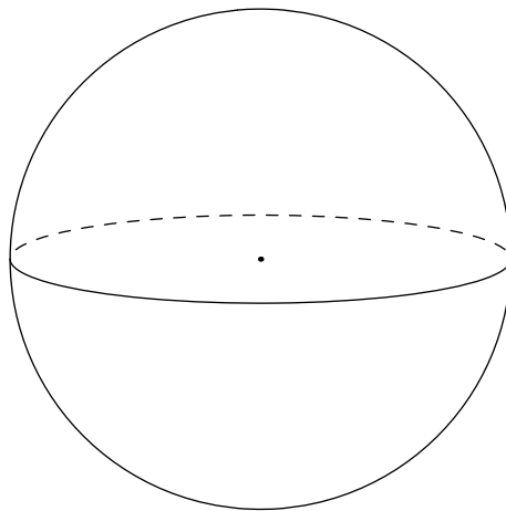
FIGURE 28.5 – Sphère
