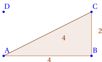
FIGURE 66.7 – Aire du triangle rectangle
