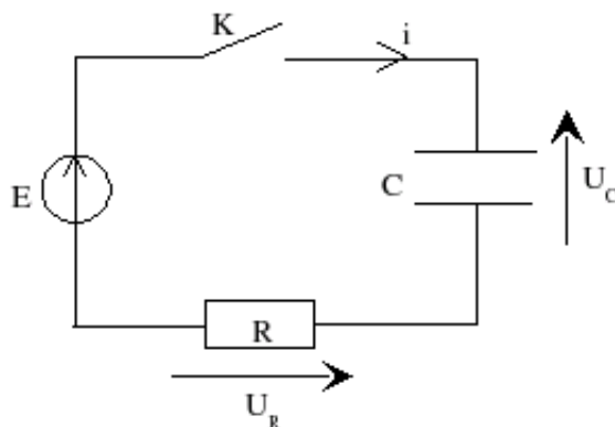
FIGURE 70.4 – Circuit RC
