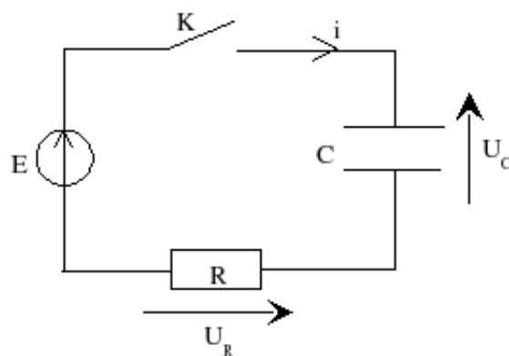
FIGURE 58.2 – Circuit RC
