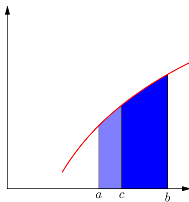
FIGURE 55.5 – Relation de Chasles
