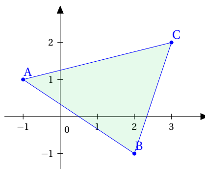
FIGURE 23.9 – Le triangle ABC
