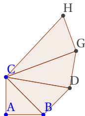
FIGURE 33.1 – Escargot
