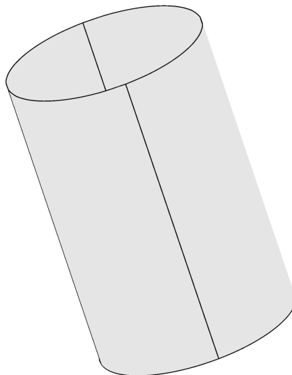
FIGURE 28.6 – Cylindre
