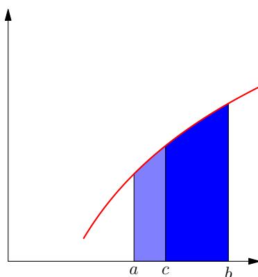
FIGURE 66.14 – Relation de Chasles
