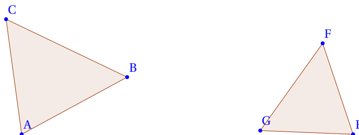
FIGURE 66.3 – Aires multiples
