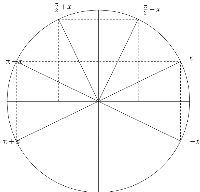
FIGURE 32.5 – Angles associés
