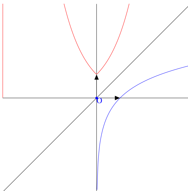
FIGURE 53.1 – Croissances comparées
