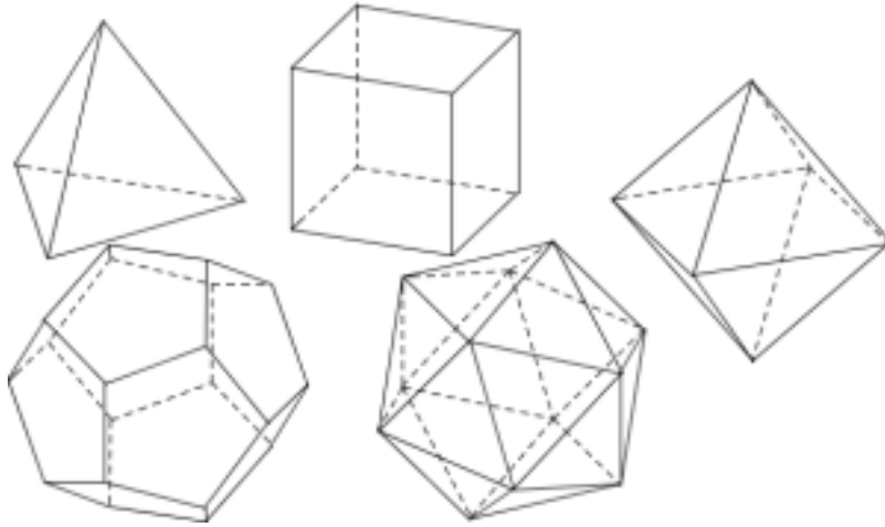
FIGURE 28.8 – Solides de Platon
