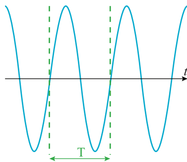
Figure 11.3 – Signal d'un diapason
