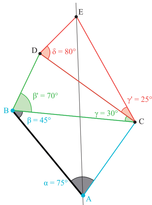
Figure 8.9 – Figure de triangulation d'une distance
