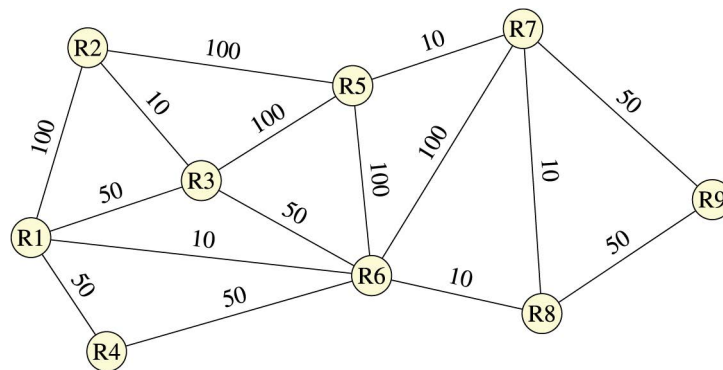
Figure 9.11 – Graphe pondéré
